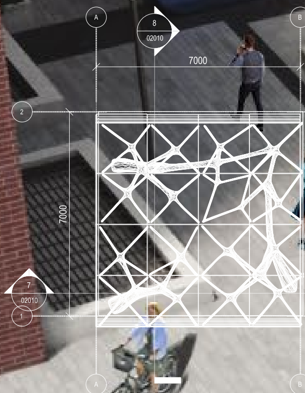
2 GARDEN PAVILION - ROOF PLAN 1:100@A1
