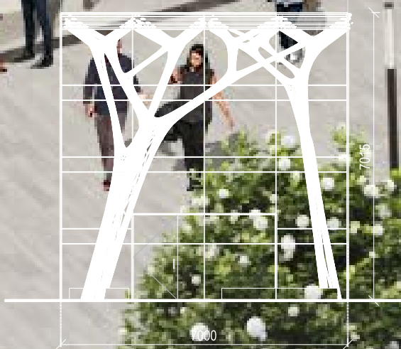
4 GARDEN PAVILION - SOUTH ELEVATION 1:100@A1
